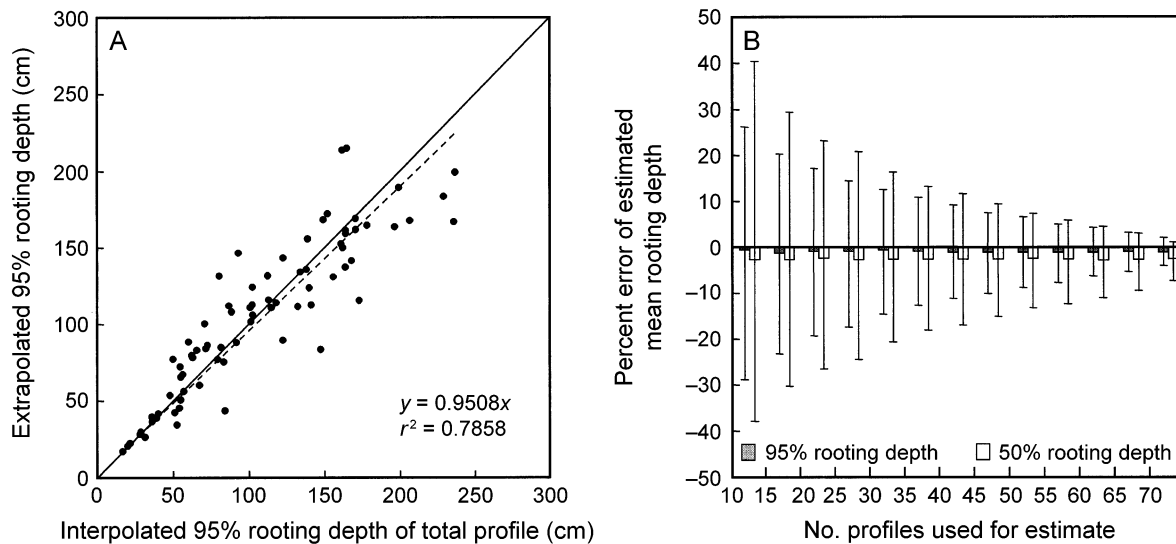
FIG. 2. (A) Comparison between 95% rooting depths estimated by extrapolation of the upper part of the root profile ( \sim 1 m depth) and 95% rooting depths interpolated for entire profiles. The data set used for this comparison consisted of 76 completely sampled test profiles. (B) Combined interpolation and extrapolation errors (%) for estimates of mean extrapolated rooting depths as a function of sample size. The error bars represent 95 percentiles of 1000 bootstrapped recalculations of mean rooting depths using subsamples of between 10 and 70 profiles.
