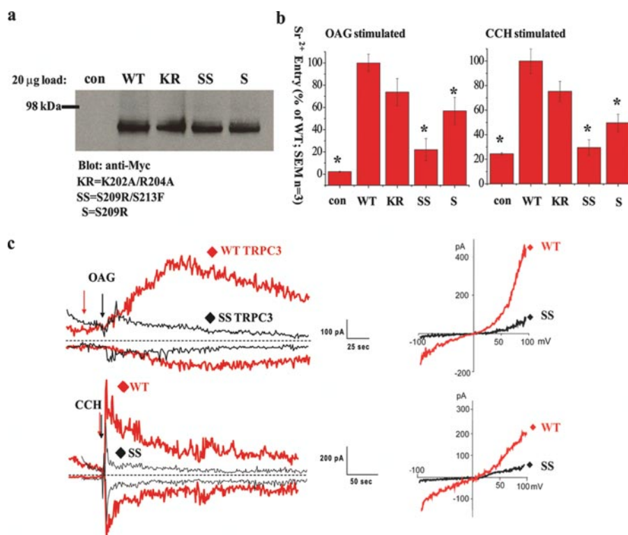
FIGURE 2. Mutations in TRP 2 disrupt channel activity. a , Western analysis of HEK293 cell lysates transfected for 24 h with either YFP alone (con) or YFP + full-length WT, K202A/R204A (KR), S209R/S213F (SS), or S209R (S) TRPC3 mutants blotted with anti-Myc antibody. b , quantification of the area under the curve for Sr 2+ entry in the presence of 100 μM OAG or 100 μM CCH stimulation in HEK293 cells transfected with either YFP alone (con) or YFP + full-length WT, K202A/R204A, S209R/S213F, or S209R TRPC3 mutants (S.E., n = 3, * p value < 0.01, Student's t test) (see supplemental Fig. S1, a and b for traces). c , whole cell electrophysiological recordings in HEK293 cells transfected with either full-length WT (red) or SS (black) TRPC3 and stimulated with 100 μM OAG or 100 μM carbachol.
